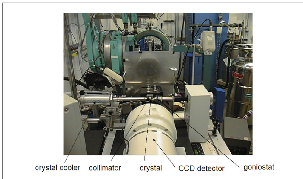
Figure 7.13.23 Inside a Synchrotron experimental station. The Marresearch charge-coupled device detector (MARCCD 225; foreground, http://www.rayonix.com ) mounted on the MAR desktop beamline (DTB) at the insertion device beamline (5-ID-D hutch) of the DuPont-Northwestern-Dow collaborative access team (DND-CAT), located at sector 5 of the Advanced Photon Source (APS). The view is into the beam that is transported along the tube visible in the center of the upper half of the photograph. The instrumentation colored light blue in the background is not part of the macromolecular crystallography setup. Work conducted at the DND-CAT now focuses more on surface and interface science, nano-materials, catalysis, and environmental science. The macromolecular crystallography efforts have moved to the new Life Sciences (LS-CAT) at sector 21 of the APS that offers four ID lines and is jointly run by Michigan institutions, Northwestern University, the University of Illinois at Urbana-Champaign, the University of Wisconsin, and Vanderbilt University. Further consortia that operate ID and/or Bending Magnet (BM) beamlines for macromolecular crystallography at the APS include BioCARS-CAT (sector 14), IMCA-CAT (sector 17), SBC-CAT (sector 19), SER-CAT (sector 22), GM/CA-CAT (sector 23), NE-CAT (sector 24), and LRL-CAT (sector 31).
