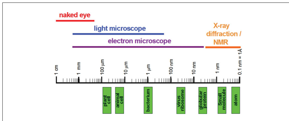
Figure 7.13.3 From the visible to the invisible. The diagram depicts the rough sizes of cells and their components on a logarithmic scale and illustrates the range of objects that can be visualized with different techniques.
