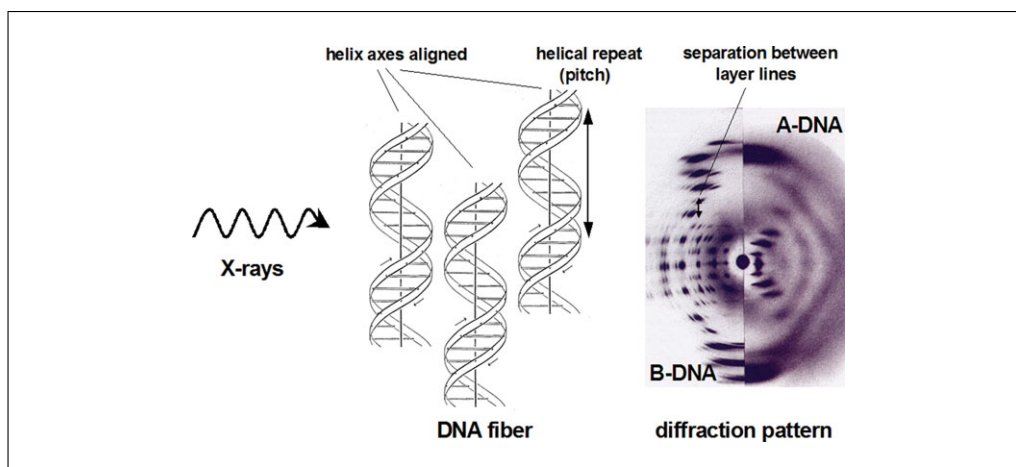
Figure 7.13.6 Principles of fiber diffraction. The diffraction pattern resulting from aligned helical structures in fibers exposed to X-rays exhibit characteristic cross-like shapes. The drawing of the DNA duplex was originally created by Odile Crick and is adapted from Kemp (2003) with permission from Nature Publishing Group.
