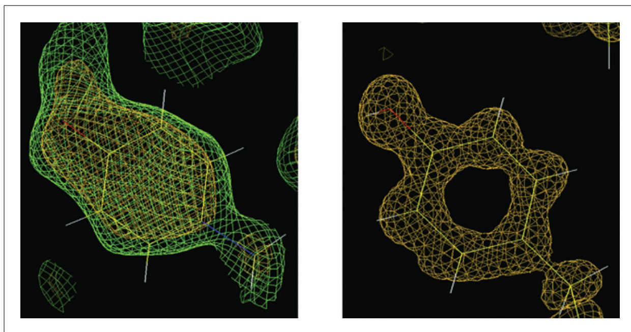
Figure 7.13.13 Neutron versus X-ray macromolecular crystallography. Left: The neutron density for Tyr137 in the structure of D-xylose isomerase contoured at 1.5\sigma (green) and 2.0\sigma (yellow) clearly reveals the orientation of the deuterium on the O atom of tyrosine. Right: The protonation state of Tyr254 remains unclear from electron density maps in the X-ray crystal structure of the same enzyme determined to 0.94-Å resolution at -170^\circ\text{C} . Reprinted from Hanson et al. (2004) with permission from the International Union of Crystallography.
