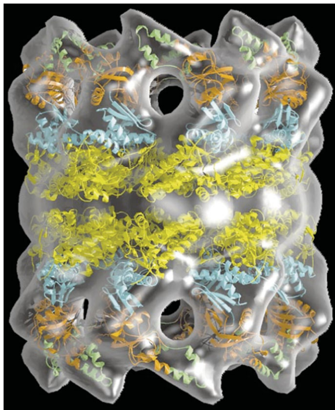
Figure 7.13.12 3D model of the archaeal thermosome holoenzyme. Crystal structures of the subunits (in color) are modeled into the EM-molecular envelope of the hexadecameric chaperone. Reprinted from Baumeister and Steven (2000) with permission from Elsevier.
