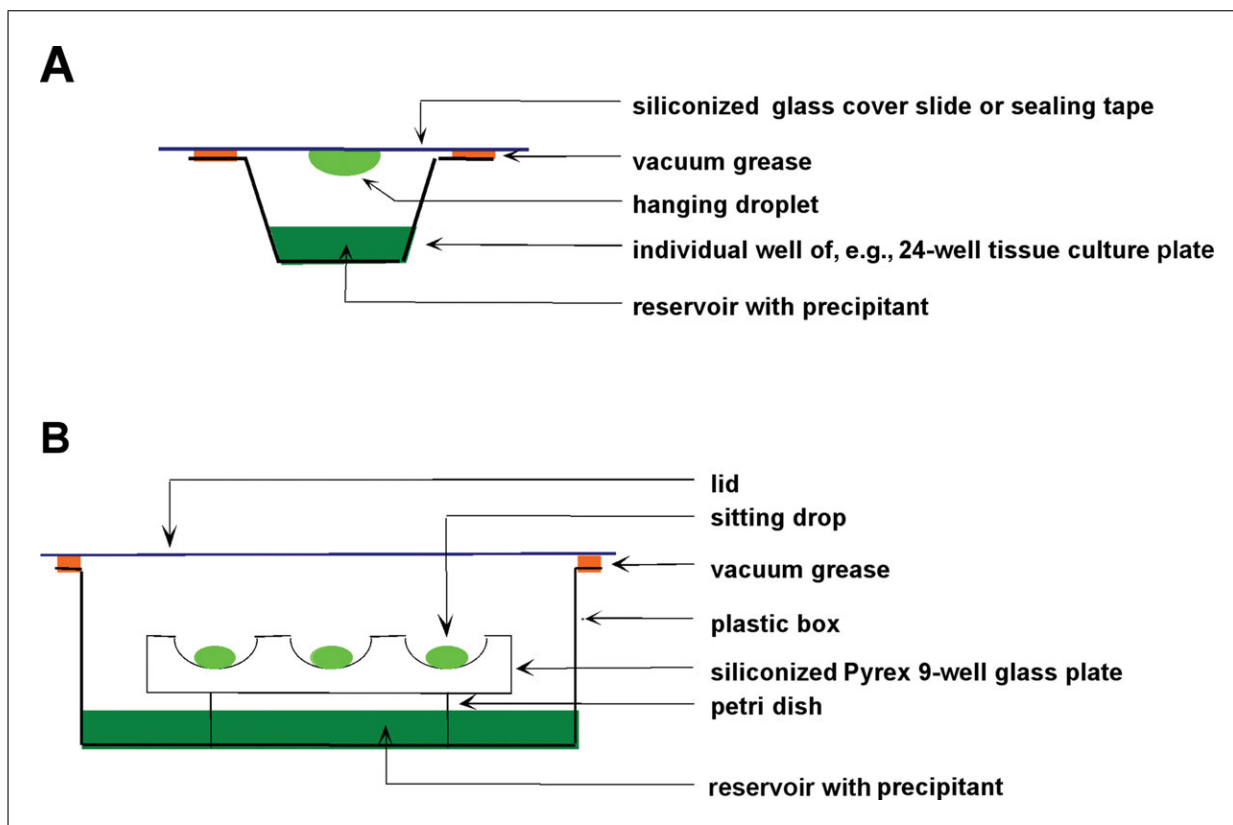
Figure 7.13.18 Two related methods for growing single crystals of biomacromolecules. Schematic depictions of the (A) hanging and (B) sitting drop vapor diffusion techniques. The volume of the droplets is in the nL (nanodrop setting robots) to \mu\text{L} range.
