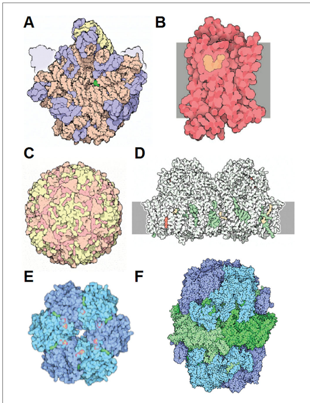
Figure 7.13.1 Recent triumphs of structural biology. (A) The ribosome (large subunit; PDB entry code 1ffk). (B) Adrenergic receptor (GPCR; PDB entry code 2rh1). (C) Poliovirus (PDB entry code 2plv). (D) Photosystem II (PDB entry code 1s5l). (E) Cyanobacterial master clock protein KaiC (PDB entry code 2gbl). (F) Fatty acid synthase (PDB entry codes 2uvb and 2uvc). Reproduced from Molecule of the Month Illustrations ( info@rcsb.org ; http://www.rcsb.org/pdb/static.do?p=education_discussion/molecule_of_the_month/index.html ) by David S. Goodsell with permission from RCSB Protein Data Bank (PDB).
