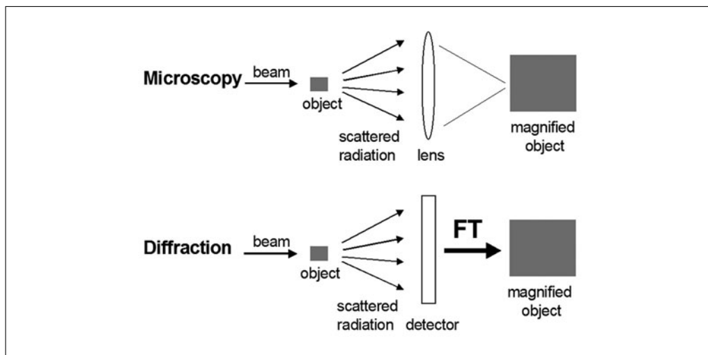
Figure 7.13.5 Light microscopy versus diffraction. Structure determination by X-ray diffraction entails the use of a mathematical lens, Fourier Transformation (FT), to “focus” the scattered radiation.
