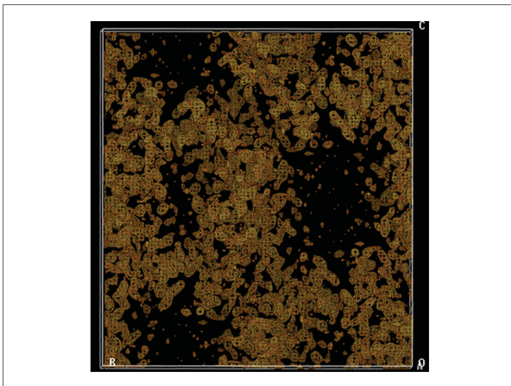
Figure 7.13.26 MAD phasing. Experimental electron density map based on five Se sites obtained from a Se-Met crystal of the Maf protein (2.7 Å resolution, no solvent flattening), calculated with the program SOLVE (Terwilliger and Berendzen, 1999). The map displays clear boundaries and reveals large solvent-filled channels (black regions).
