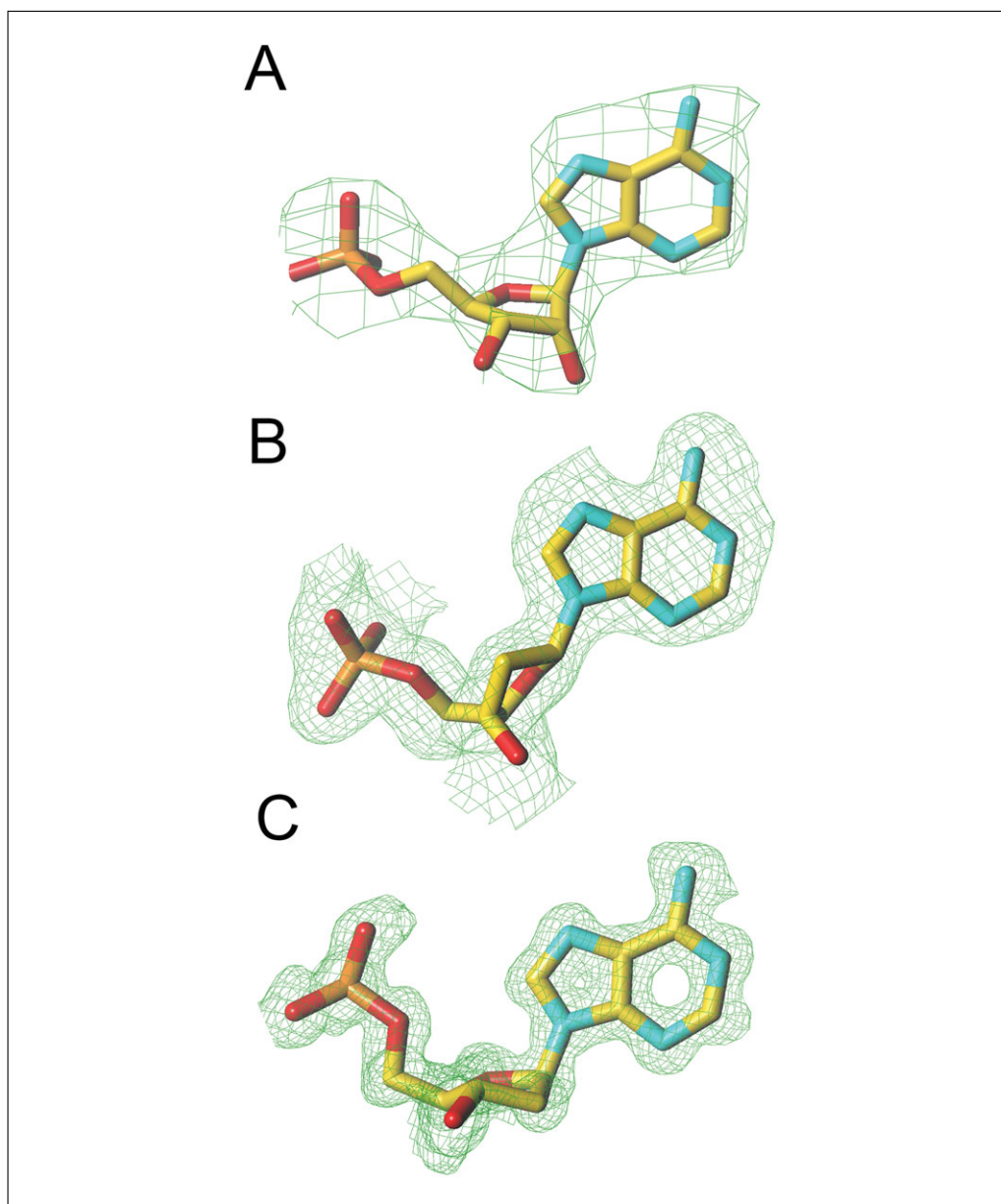
Figure 7.13.27 Resolution and quality of the electron density. Comparison of the quality of the Fourier ( 2F_o - F_c ) sum electron density around adenosine monophosphate in crystal structures obtained at various resolutions ( 1\sigma threshold). (A) 2.85 Å, ATP in the crystal structure of the KaiC protein from Synechococcus elongatus . (B) 1.80 Å, A residue in the crystal structure of a B-form DNA. (C) 1.10 Å, atomic resolution, A residue in the crystal structure of an A-form DNA.
