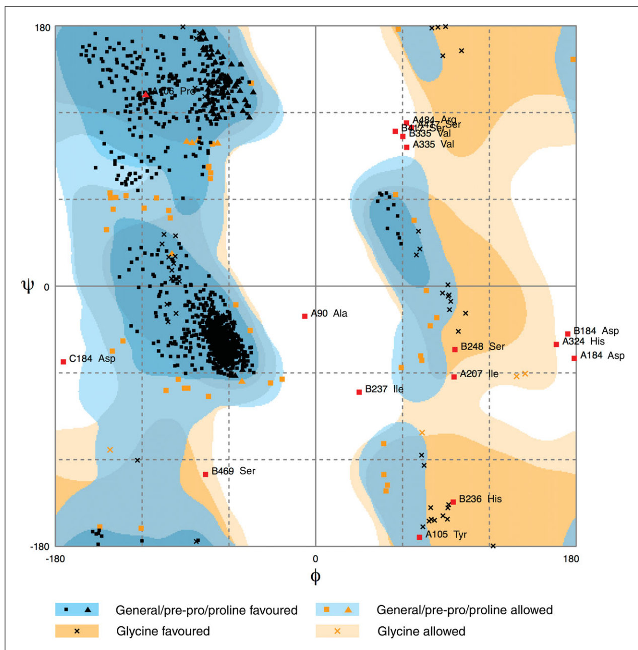
Figure 7.13.28 Structure refinement and quality control. Conformations of the \Phi and \Psi backbone torsion angle pairs (Ramachandran plot) for amino acids in the crystal structure of human cytochrome P450 21A2 in complex with progesterone (PDB ID code 4Y8W; Pallan et al., 2015). Individual angles fall either into the preferred regions (1230 residues [94.5%]) or allowed regions (44 residues [3.4%]), and the rest are outliers (red squares). The plot was generated with RAMPAGE ( http://mordred.bioc.cam.ac.uk/~rapper/rampage.php ; Lovell et al., 2003).
