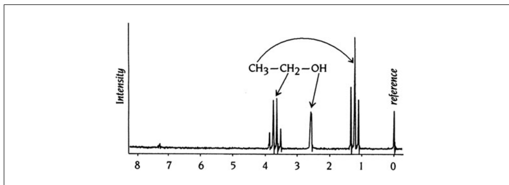
Figure 7.13.15 One-dimensional ^1\text{H} -NMR spectrum of ethanol. The three groups of protons in this small molecule, (\text{C})\text{H}_3 , (\text{C})\text{H}_2 , and (\text{O})\text{H} , all exhibit different chemical shifts relative to the protons in reference molecule, tetramethylsilane (TMS). The characteristic splitting of the signals arising from the methyl (1:2:1) and methylene (1:3:3:1) protons is the result of through-bond coupling between neighboring nuclei.
