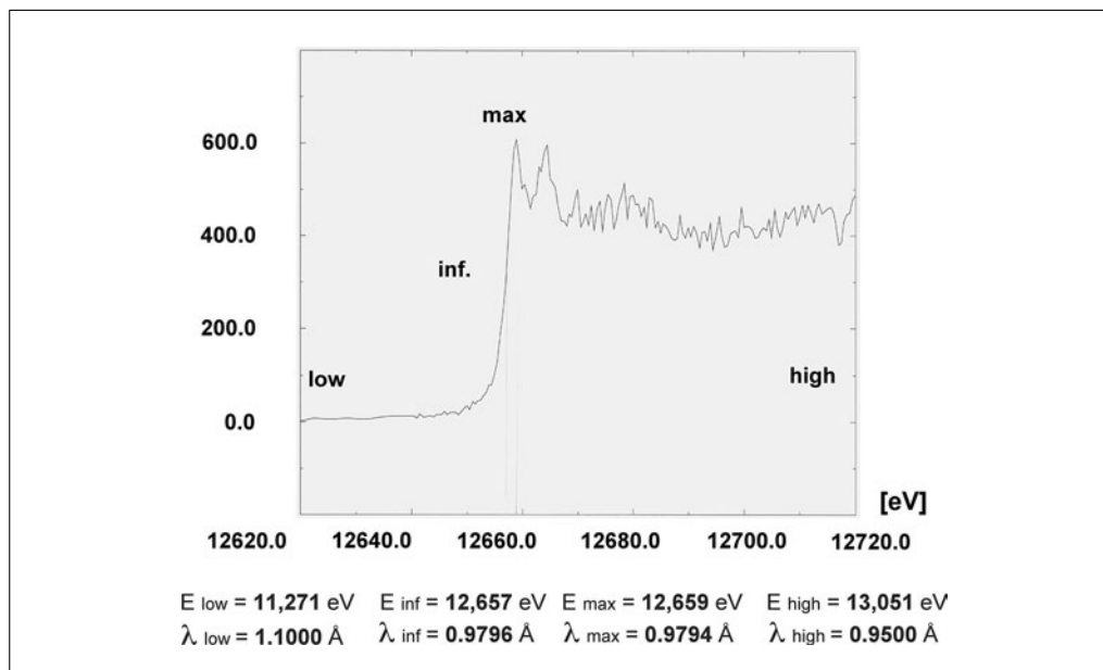
Figure 7.13.25 Multiwavelength anomalous dispersion (MAD) experiment. Example of an X-ray fluorescence spectrum from a protein crystal that contains Se-methionine (Se-Met) in place of Met (Maf protein from Bacillus subtilis ; 189 amino acids and 6 Se atoms per protein molecule). The theoretical K absorption edge of selenium lies at 12.6578 keV or 0.9795 Å (an energy of 12.398 keV corresponds to 1.0 Å; http://skuld.bmsc.washington.edu/scatter/ ). In a typical MAD experiment, diffraction data of high redundancy from the same crystal are collected at three or four wavelengths (i.e., reference below the edge, low, inflection point, inf., peak, max, and reference above the edge, high).
