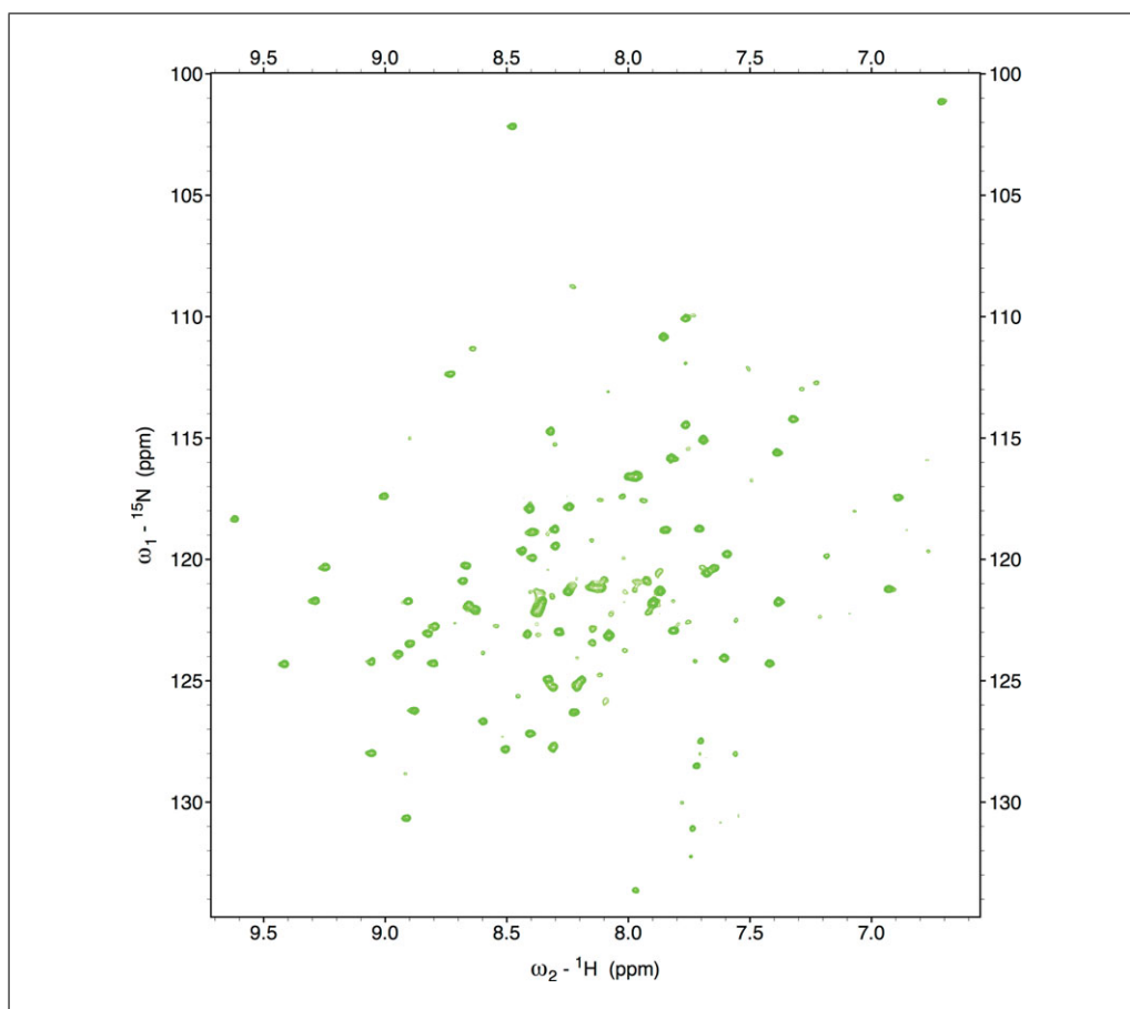
Figure 7.13.16 Two-dimensional heteronuclear NMR spectroscopy. ^{15}\text{N} -HSQC spectrum of the circadian clock protein KaiB from the cyanobacterium Synechococcus elongatus recorded on an 800-MHz spectrometer. HSQC, heteronuclear single quantum correlation.
