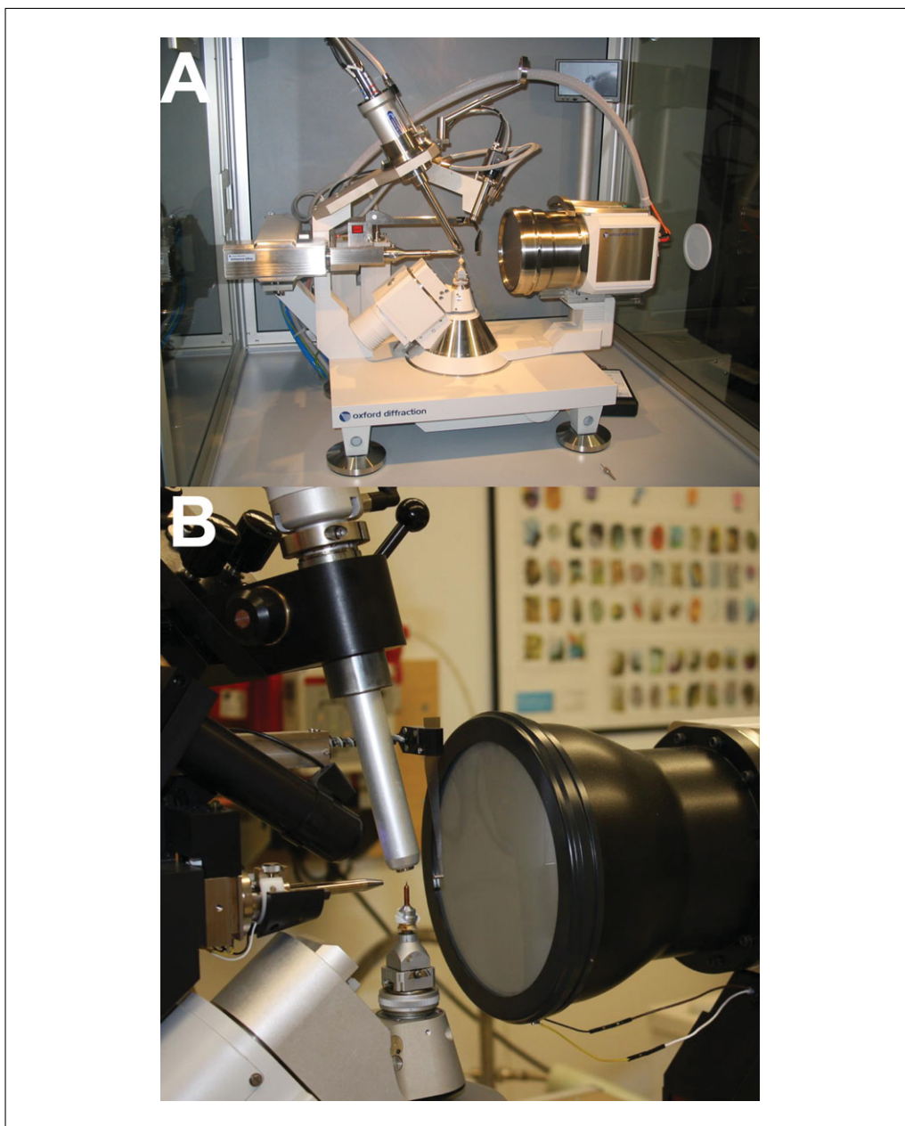
Figure 7.13.21 X-ray generators and detectors. Two 4-circle, kappa-geometry X-ray diffraction setups currently used by researchers at Vanderbilt University. (A) The sealed tube Oxford Xcalibur PX2 Ultra (Oxford Diffraction). (B) The rotating anode Bruker Microstar (Bruker AXS). Tube housing (Xcalibur), beam collimator, beam stop, CCD detector, crystal cooler, goniostat, goniometer head, and telescope are clearly visible.
