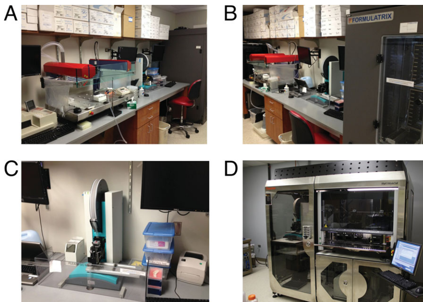
Figure 7.13.20 Automation of crystallization experiments. Crystallization robotics at Vanderbilt University include: (A) A Xantus lipidic cubic phase robot. (B) A Formulatrix Rock Imager for storage and automatic imaging of crystallization plates. (C) A TPP LabTech Mosquito nanodrop setter robot. (D) In the laboratory of the author, the MaX WorkCell by Thermo Fisher Scientific. The WorkCell integrates nanodrop setting (“Mosquito,” on the left), liquid handling, and screen preparation (“Starlet,” Hamilton Company; on the right), and sealing of crystallization plates (bottom right).
