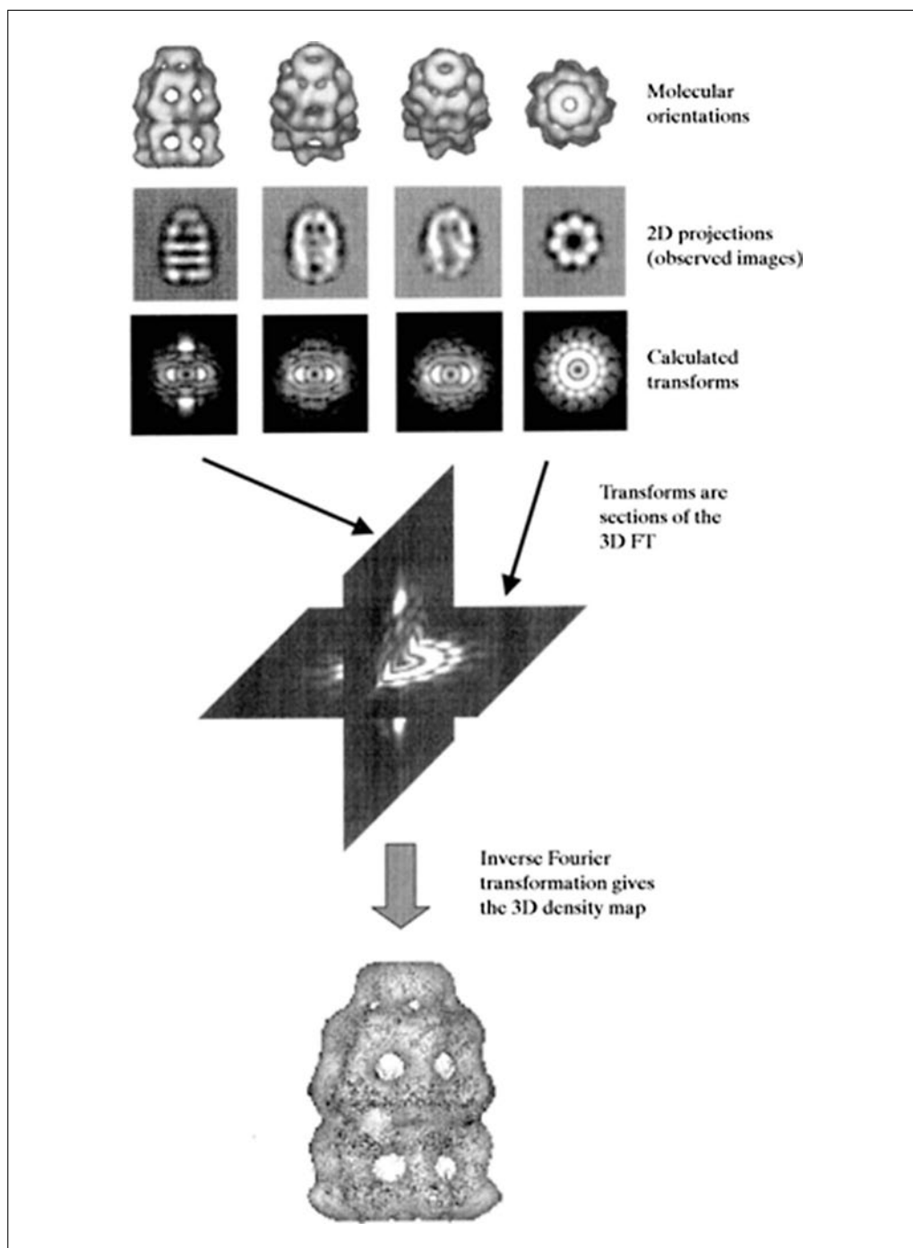
Figure 7.13.10 Single-particle electron microscopy (EM) 3D-reconstruction from 2D-projections. A set of 2D-projections (four in this case) is depicted along rendered iso-surfaces. The Fourier transform (FT) of a 2D-projection is equivalent to a central section in the 3D-FT of a molecule. Once a sufficient number of sections are available, the complete 3D-transform can be generated and inverse-transformed into a 3D-density map (bottom). Reprinted from Saibil (2000) with permission from the International Union of Crystallography.
