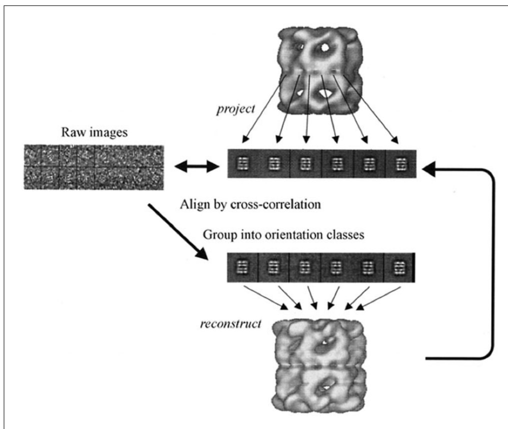
Figure 7.13.11 Refinement by projection matching. Reference images are created by projecting a 3D-map into a set of different orientations (center). Each raw image from the data set (left) is then rotationally and translationally aligned to individual reference images and given the orientation with the highest correlation coefficient. Images aligned in this fashion are grouped and averaged once again to create an improved 3D map (bottom). Reprinted with permission from Saibil (2000) with permission from the International Union of Crystallography.
