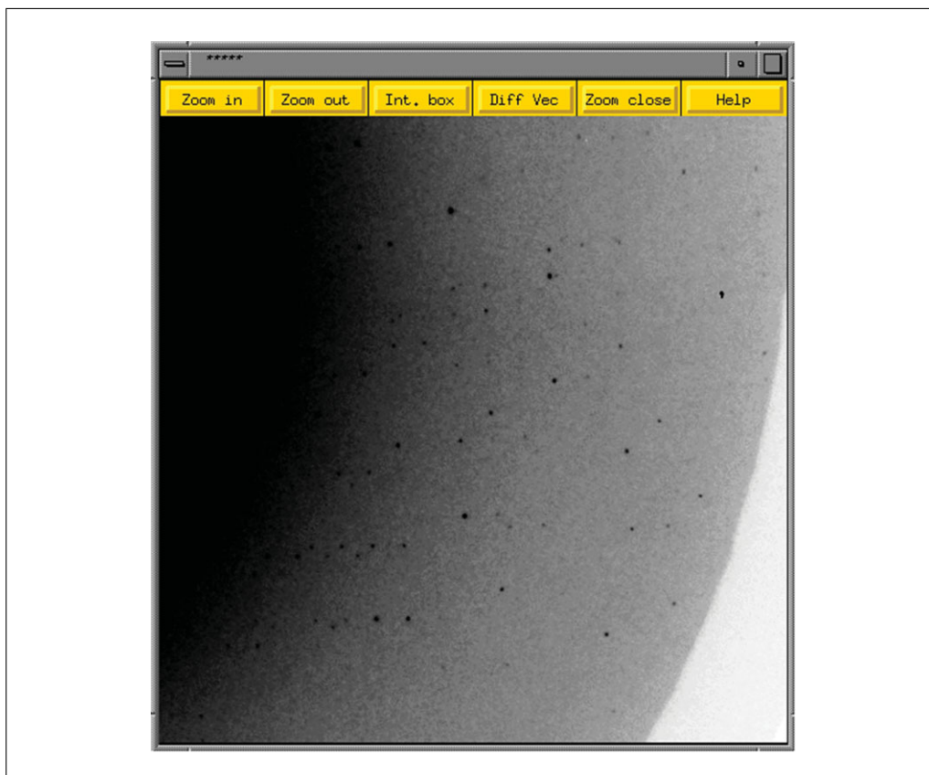
Figure 7.13.24 Diffraction data collection. Close up of a 1^\circ ( \Delta\Phi ) diffraction image obtained from a single crystal of the so-called Dickerson Drew Dodecamer (DDD; B-form DNA of sequence CGCGAATTCGCG). The dark spots represent individual reflections and the diffraction limit is around 1 \text{ \AA} . Data statistics for this particular crystal of the DDD are listed in Table 7.13.5.
