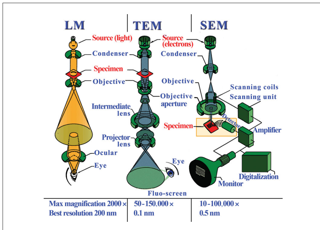
Figure 7.13.7 Light microscopy versus electron microscopy. Lenses allow reconstruction of the image in both techniques, but to focus electron beams electromagnetic lenses are required. Standard light microscope (LM, left), transmission electron microscope (TEM, center), and scanning electron microscope (SEM, right). Source: http://www.vcbio.science.ru.nl/images/fesem_beam_zoom.jpg . Original illustration: Jeol Instruments. Redrawn by vcbio.science.ru.nl, Radboud University Nijmegen. Used with permission.
