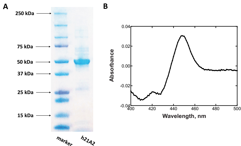
FIGURE 3. Purification of human P450 21A2. A, SDS-PAGE. The molecular weight marker (left) and purified P450 21A2 (right) are indicated. B, \text{Fe}^{2+}\cdot\text{CO} versus \text{Fe}^{2+} difference spectrum ( 0.38 \mu\text{M} P450) (28). (Safranin T ( 1 \mu\text{M} ) was added as an electron mediator (29).)
