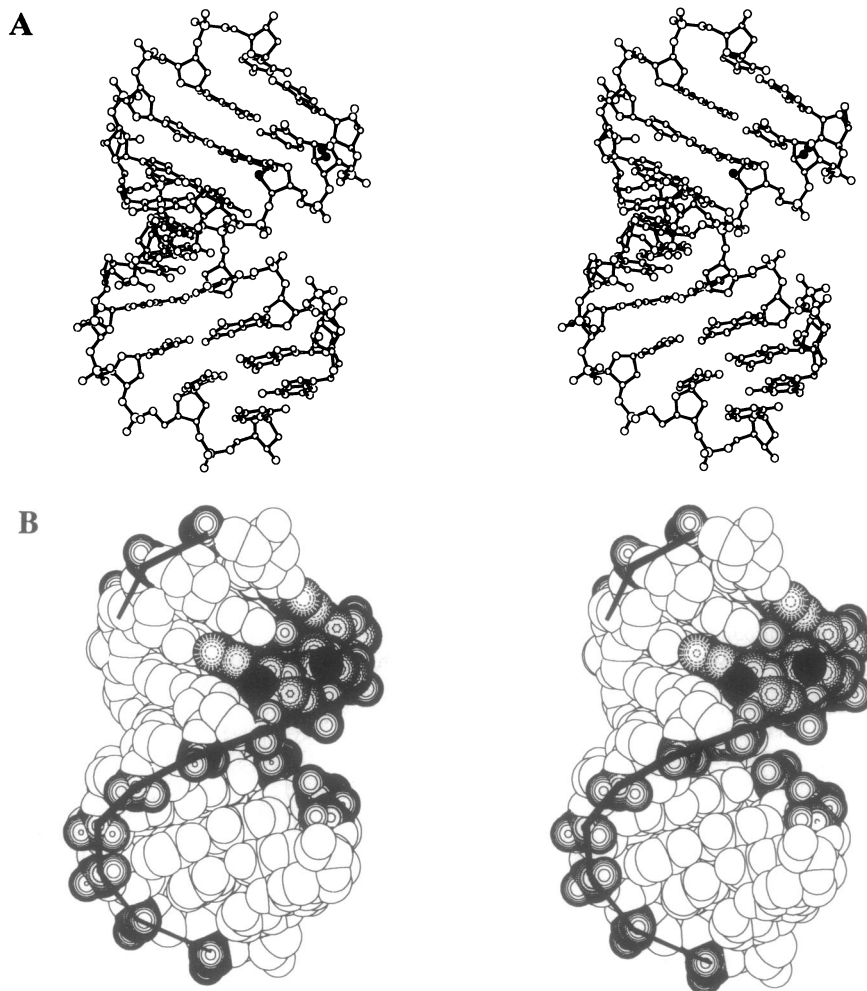
FIG. 4. (A) Stereo skeletal drawing of the Okazaki fragment (minor groove on the left and major groove on the right). The RNA primer (to the upper right) is drawn with solid bonds and the DNA is drawn with open bonds. The DNA strand dG(1) to dC(10) runs from the upper right to the lower left; the chimeric RNA-DNA strand rG(11) to dC(20) runs from the upper right to the lower left. Atom types are coded according to size with P > O > N > C and O2' oxygens are solid. (B) Stereo van der Waals representation of the Okazaki fragment (view identical to A). Darker patterns highlight RNA atoms (carbons, wavy circles; oxygens, concentric circles; nitrogens, dashed circles; O2' oxygens, solid black) and phosphorus groups are traced with solid lines to emphasize the backbones. Note that only the O2' oxygens of residues rC(12) and rG(13) are lying at the surface of the minor groove and that the O2' oxygen of residue rG(11) is located in the major groove and, therefore, is hidden.
