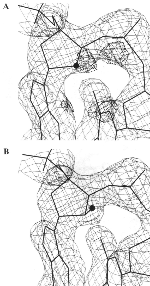
FIG. 3. (A) Sum and difference ( F_{\text{obs}} - F_{\text{calc}} ) density around the ribose of residue rG(13), before addition of the \text{O}2' oxygen ( R -factor, 19%; 2 \text{ \AA} data). The \text{C}2' carbon is highlighted with a large dot. The superimposed sum (thin lines) and difference densities (dashed lines) around \text{C}2' indicate the missing \text{O}2' oxygen [residue rC(12) is similar]. (B) Identical to view in A, showing the sum density after the final refinement steps (no difference density is present at the same display level as in A). The position of the \text{O}2' oxygen is highlighted with a large dot. The densities around the \text{O}2' oxygens of residues rC(12) (visible in Fig. 2B at the very left) and rG(11) are resolved similarly.
